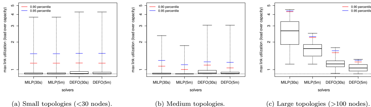
Figure 3: Max-congestion analysis results obtained with REPETITA. Top and bottom of the boxes represents 25-th and 75-th percentiles, the thick line in the boxes the median, and top and bottom whiskers minimum and maximum values, respectively. The dashed horizontal line is the theoretical lower bound, computed by REPETITA.
