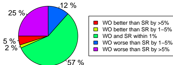
Figure 4: Systematic comparison through REPETITA between maximum link utilization induced state-of-the-art algorithms relying on weight optimization or SR.
