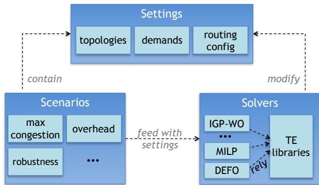
Figure 1: REPETITA architecture.
