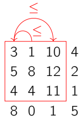
Order-preserving submatrix (OPSM) [Ben+02]
